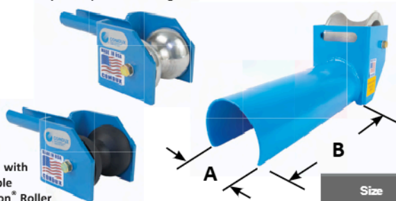
1.5" (38 mm) Cable Feeding Sheave
