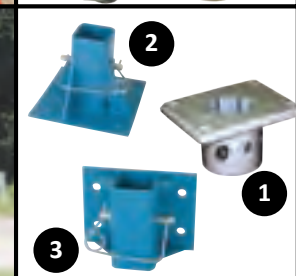
Mounting Sockets 1-Floor Socket Mount 2-Base Mount 3-Side Mount
