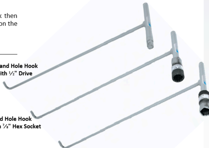
Hand Hole Hook with 7/8" Penta Socket
